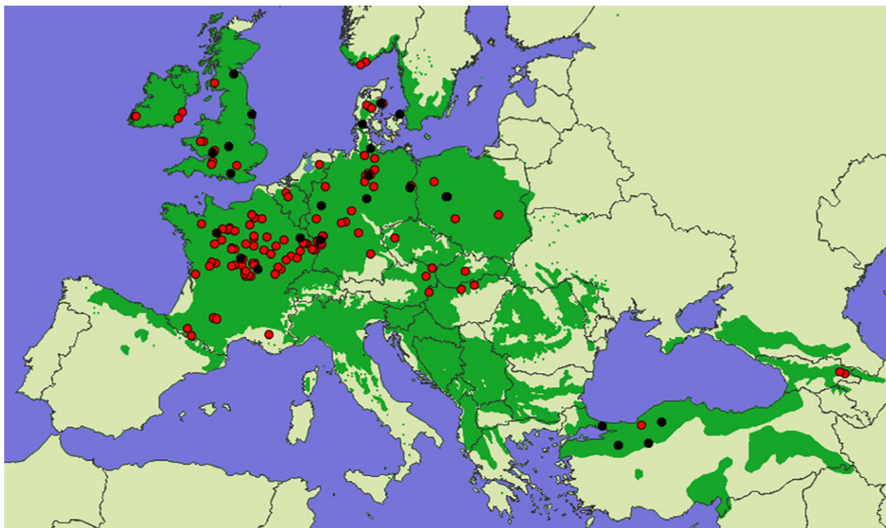
Fig. 1 Location of source populations and test sites. Red symbols indicate the locations of the 116 Quercus petraea populations from which seeds were collected for field tests. Black symbols indicate the 23 field test sites. The contemporary distribution of natural and naturalized stands is shown in dark green (EUFORGEN, 2009).
