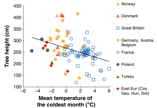
Fig. 3 Observed tree height (10-year-old trees) averaged by population, across test sites, and plotted against the mean temperature of the coldest months for the seed source (MTCM; r = -0.38 ; P < 0.0001 ). Colors indicate the country of the seed source, not the country of the test site (for eastern Europe: Cze = Czech Republic, Geo = Georgia, Hun = Hungary, Svk = Slovakia).
