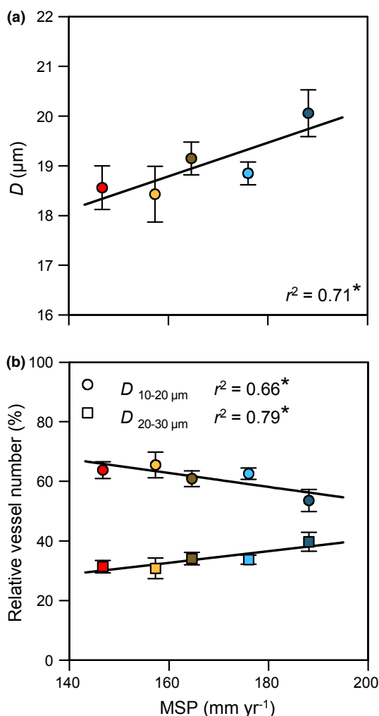
Fig. 3 (a) Vessel diameter ( D ) and (b) percentage of vessels relative to the total number of vessels diameter, classes 10–20 \mu\text{m} and 20–30 \mu\text{m} , in dependence on mean early summer growing season precipitation (MSP) in European beech ( Fagus sylvatica ). Values are mean \pm SE per site. Asterisks indicate the level of significance (*, P < 0.05 ). For explanations of symbol colours, see Table 1.
