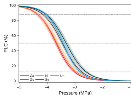
Fig. 1 Mean vulnerability curves for the five beech ( Fagus sylvatica ) forests differing in water availability showing xylem pressure in relationship to percentage loss of hydraulic conductance (PLC). The curves shown have been averaged for all samples per tree and subsequently across the five trees, 16 per site. For site abbreviations, see Table 1. The shaded band represents the SD. Different colours indicate differences in water availability.
